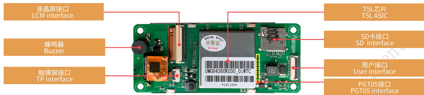
硬件接口图 Hardware interface
