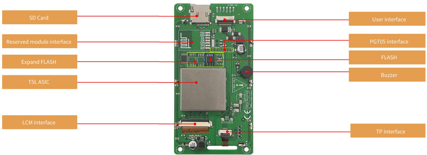
Hardware interface
