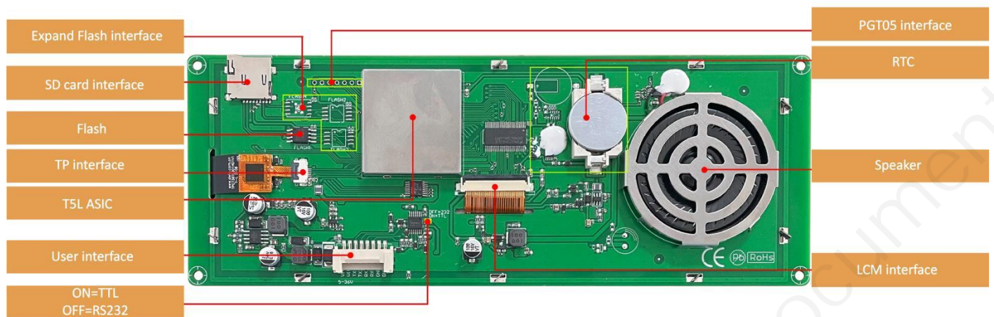
Hardware interface
