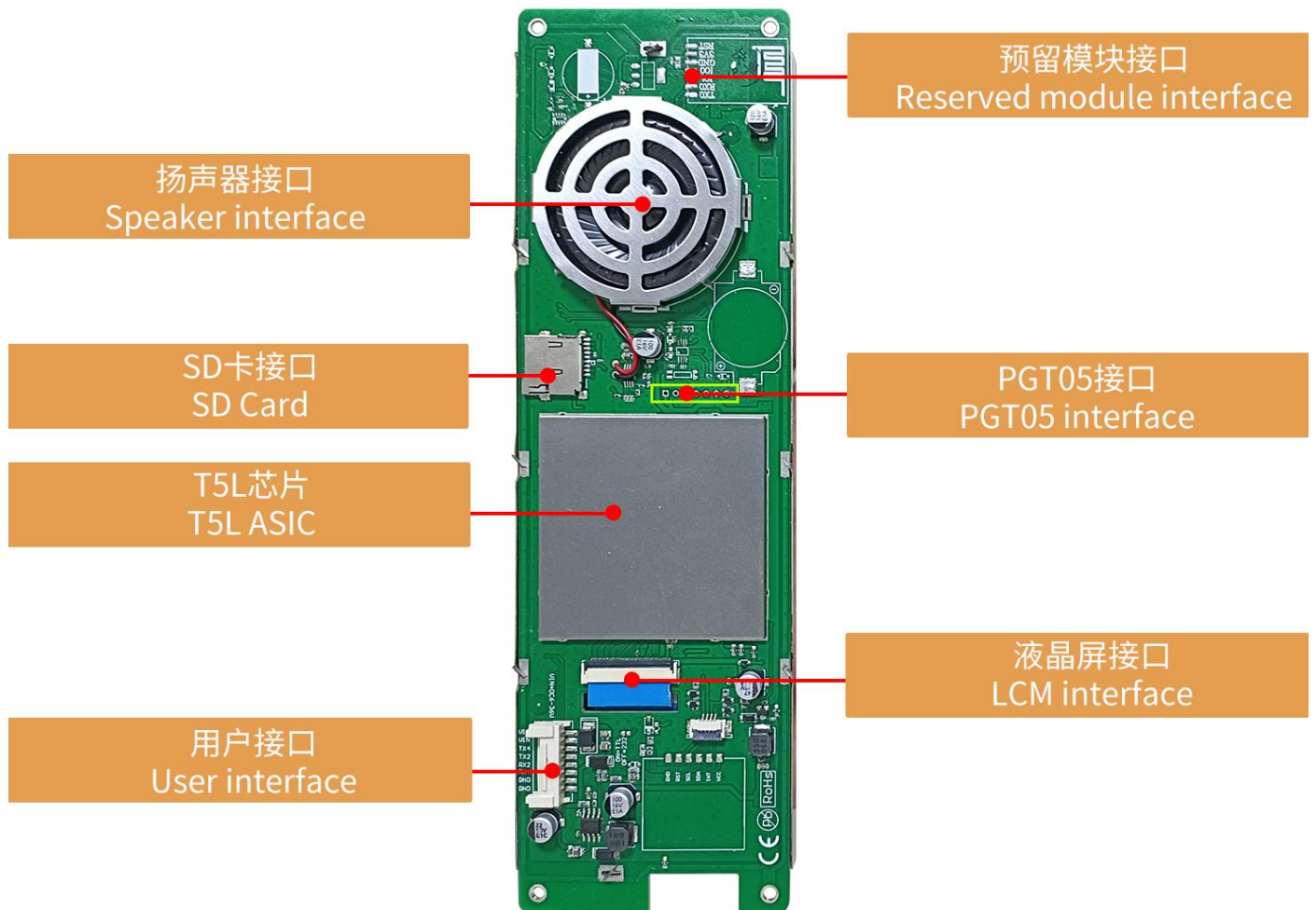
硬件接口图 Hardware interface
